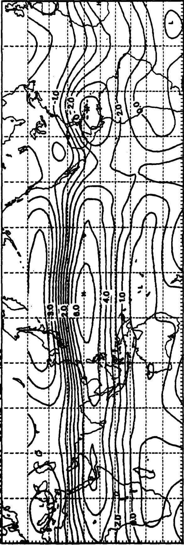
STREAM FUNCTION 200MB FEB 1983
